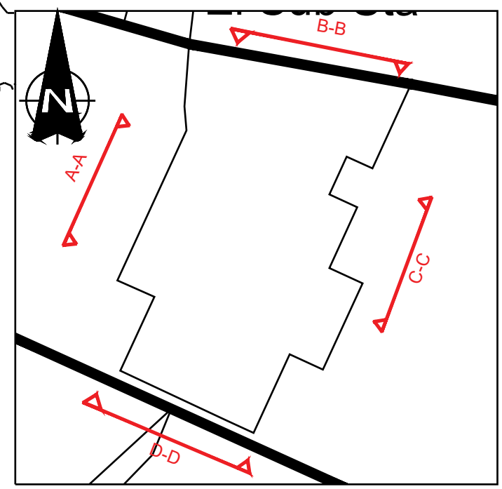
ELEVATION REFERENCE PLAN (NTS)
