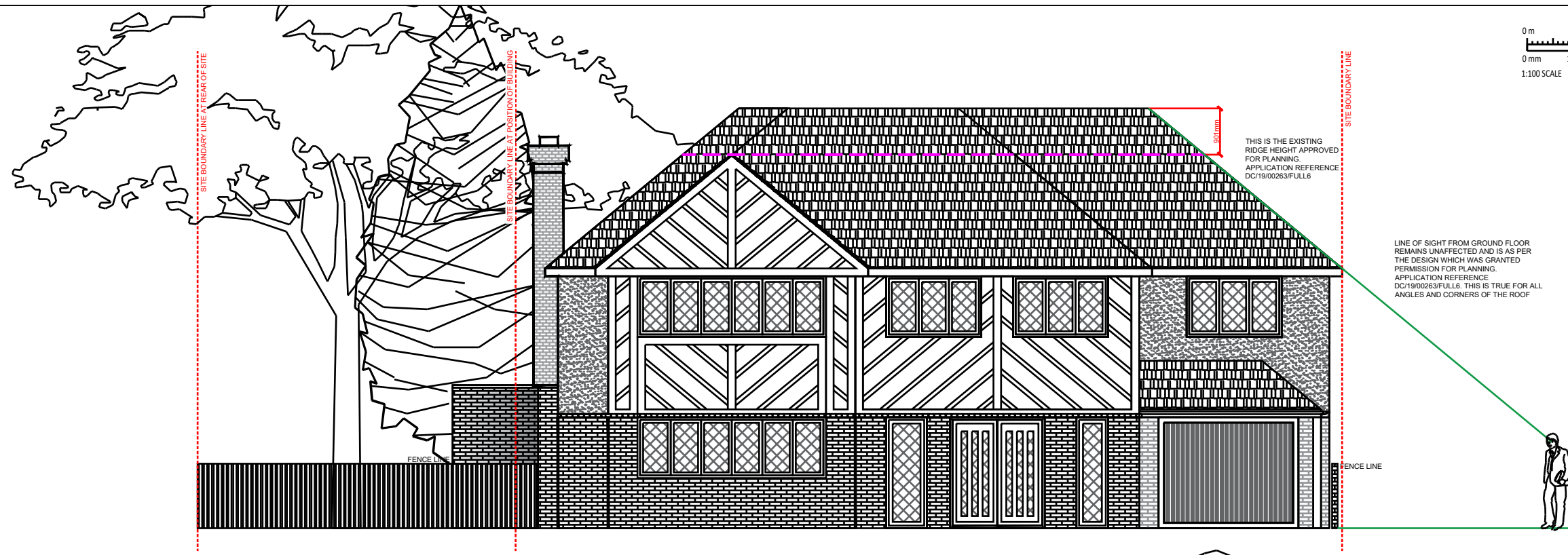
PROPOSED ELEVATION A-A
